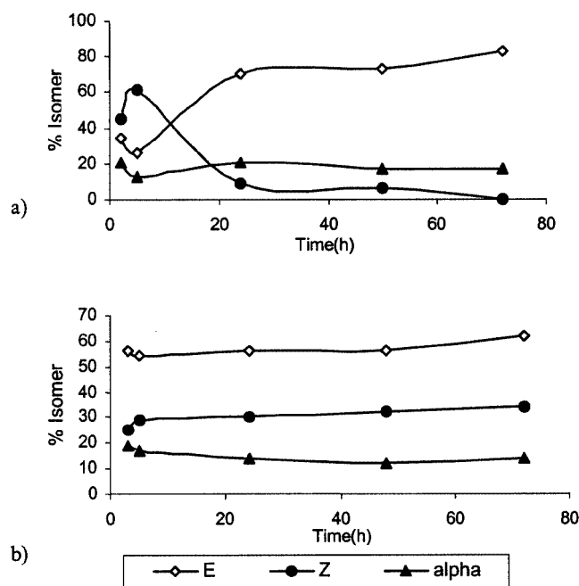
Figure 4. Reaction profiles for the hydrosilylation reactions of phenylacetylene by using 3-Me 2 (1 mol % ratio) with: (a) HSiMe 2 Ph, and (b) HSi(OEt) 3 ; percentage of isomer relative to molar fraction ( E + Z + α = 100)
