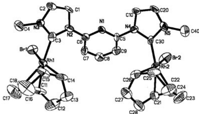
Figure 1. ORTEP diagram of 3-Me 2 with 50% probability ellipsoids; hydrogen atoms omitted for clarity; selected bond lengths (Å) and angles (°): Rh(1)–C(3) 2.029(11), Rh(1)–C(15) 2.095(12), Rh(1)–C(14) 2.105(12), Rh(1)–C(11) 2.200(12), Rh(1)–C(18) 2.220(11), Rh(1)–Br(1) 2.5172(17), Rh(2)–C(30) 1.948(11), Rh(2)–C(26) 2.101(11), Rh(2)–C(25) 2.157(12), Rh(2)–C(22) 2.189(11), Rh(2)–C(21) 2.216(11), Rh(2)–Br(2) 2.5169(18); C(3)–Rh(1)–Br(1) 87.7(3), C(30)–Rh(2)–Br(2) 90.2(3)
