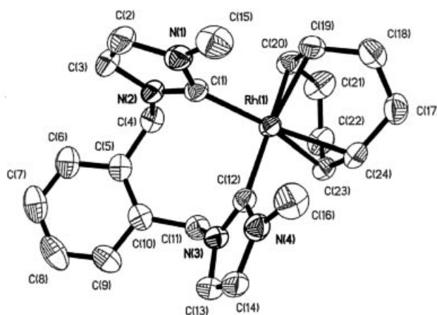
Figure 3. ORTEP diagram of 5 with 50% probability ellipsoids; hydrogen atoms omitted for clarity; selected bond lengths (Å) and angles (°): Rh(1)–C(12) 2.027(3), Rh(1)–C(1) 2.050(3), Rh(1)–C(23) 2.193(3), Rh(1)–C(19) 2.199(3), Rh(1)–C(24) 2.222(3), Rh(1)–C(20) 2.225(3); C(12)–Rh(1)–C(1) 90.55(11), C(19)–Rh(1)–C(24) 80.57(12), C(23)–Rh(1)–C(20) 80.95(12)
