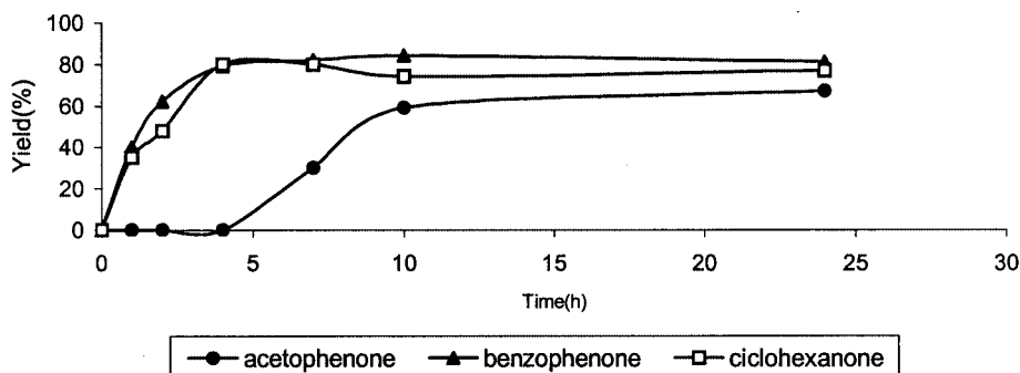
Figure 5. Reaction profile for the hydrogen-transfer reaction; 80 °C and 0.06 mol % catalyst ( 4 )
